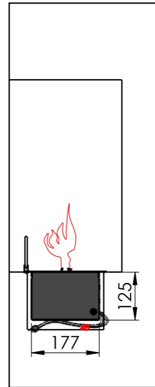
SECTION L-L
