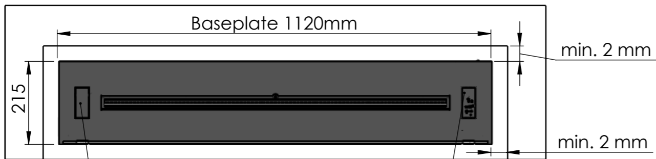
SECTION O-O
